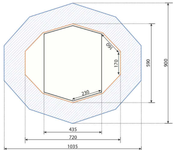
TENT WINTERIZATION MODULE FOOTPRINT
